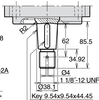
Tapered key shaft "V" SAE J744 38-3 (C-C)
