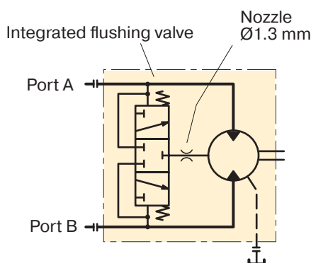
Hydraulic schematic.
