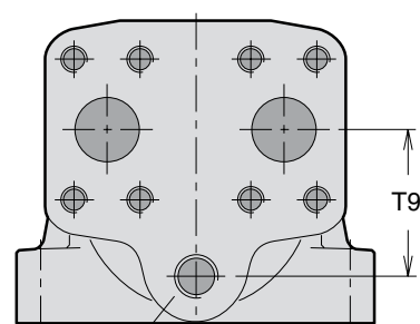
Port E (third drain port) F10-125 barrel housing (SAE version)
