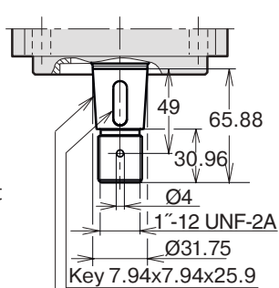
Tapered key shaft "V" SAE J744 32-3 (C)
